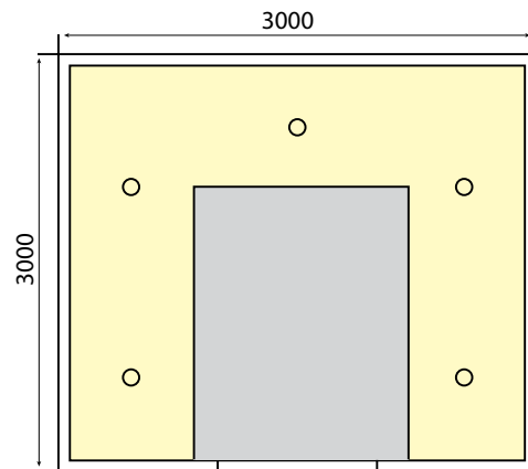
Door 800 x 1900mm 9kW Steam Generator
