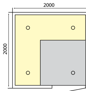
Door 800 x 1900mm 6kW Steam Generator
