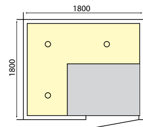
Door 800 x 1900mm 6kW Steam Generator
