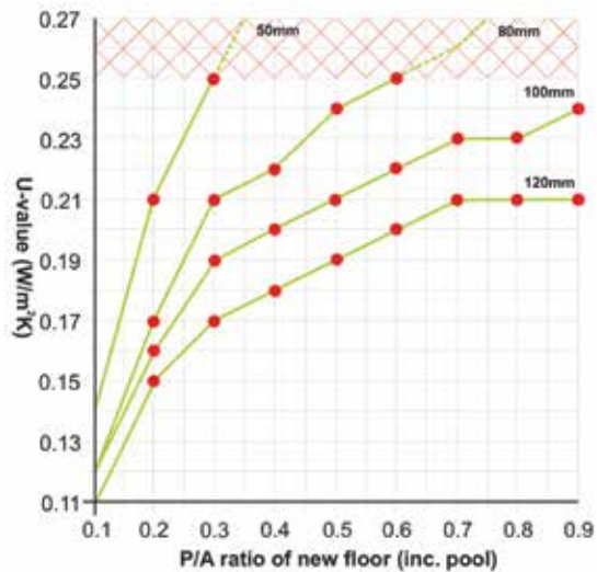
Typical Thermal Performance (Calculated in accordance with ISO 13370)
