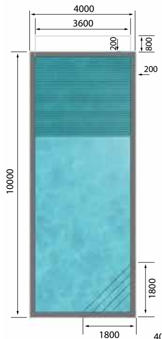
Option B - Pool with steps and Roldeck cover
