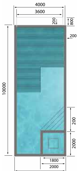
Option D - Pool with steps, Vitality Spa & Roldeck Cover
