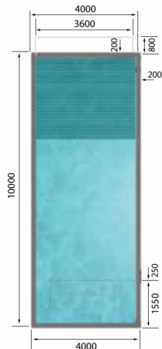
Option F - Pool with Vitality Seat, Steps & Roldeck Cover
