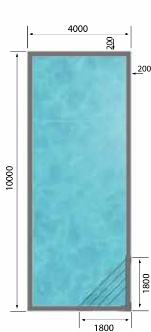
Option A - Pool with steps
